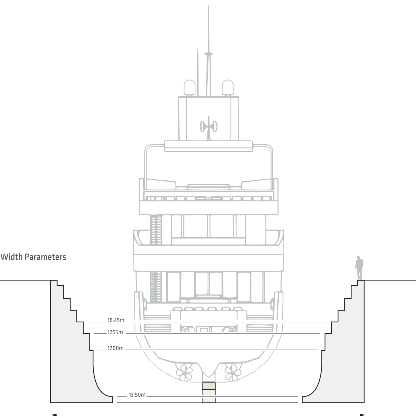
DRY DOCK 2 REAR ELEVATION
