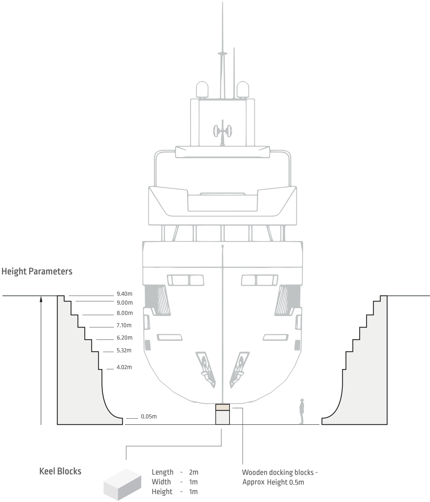
DRY DOCK 2 FRONT ELEVATION
